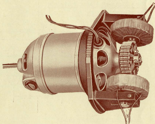
Universal Motor, complete with synchronising gear Price £7 7 0
