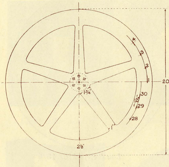
The Baird Graduated Receiving Disc PRICE £2 2s. 0d.
