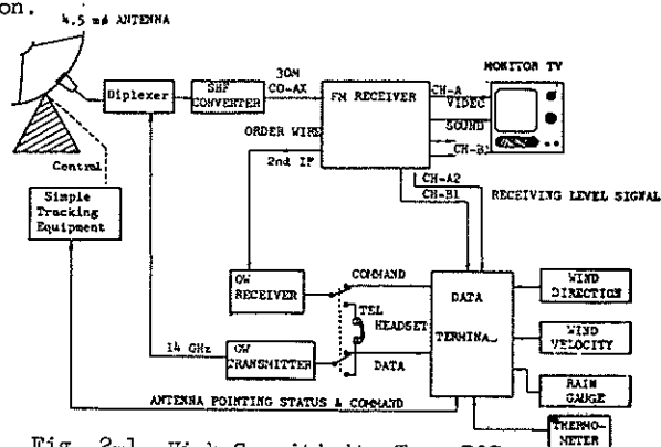
Fig. 2-1 High Sensitivity Type ROS
