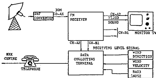
Fig. 2-2 Medium Sensitivity Type ROS
