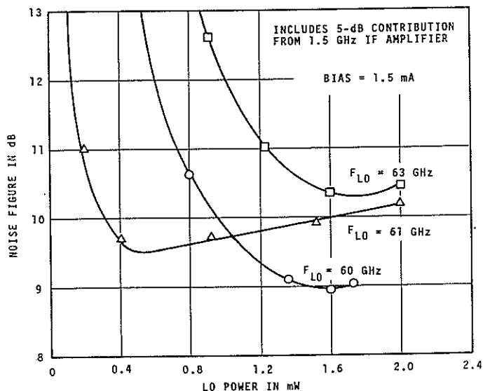
Fig. 4. Noise figure of mixer with GaAs diode.
