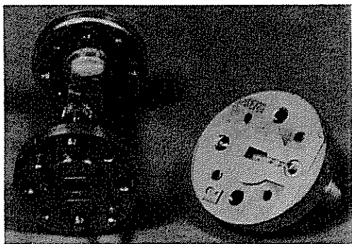
Fig. 3. Advanced mixer mount.
