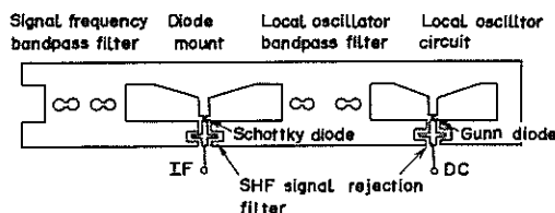
Fig. 1. Construction of 12-GHz converter with planar circuit in waveguide.
