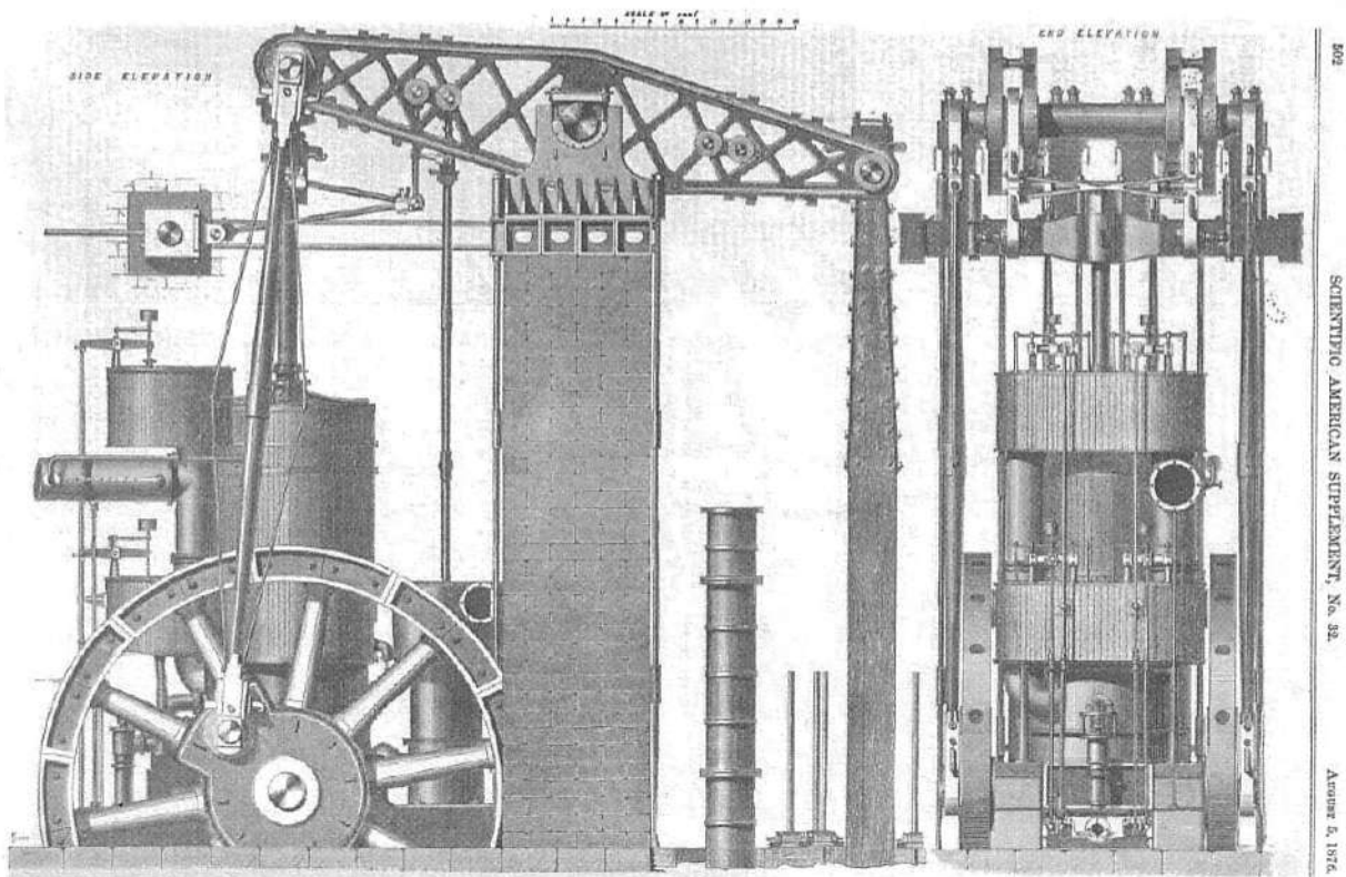
PUMPING-ENGINE OF THE LEHIGH ZINC COMPANY, PENNSYLVANIA.—(See page 504.)
