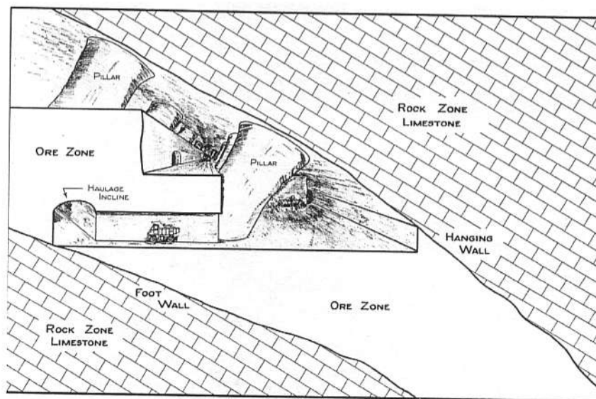
CROSS SECTION SHOWING PROPOSED MINING SYSTEM FOR FRIEDENSVILLE —LOOKING EASTERLY—
