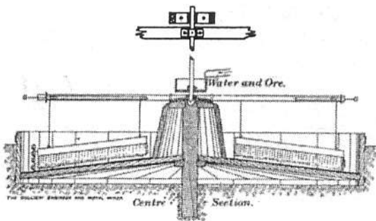
Buddle of the type used at the Friedensville mines. (From: Landis, "Zinc Mining.")
