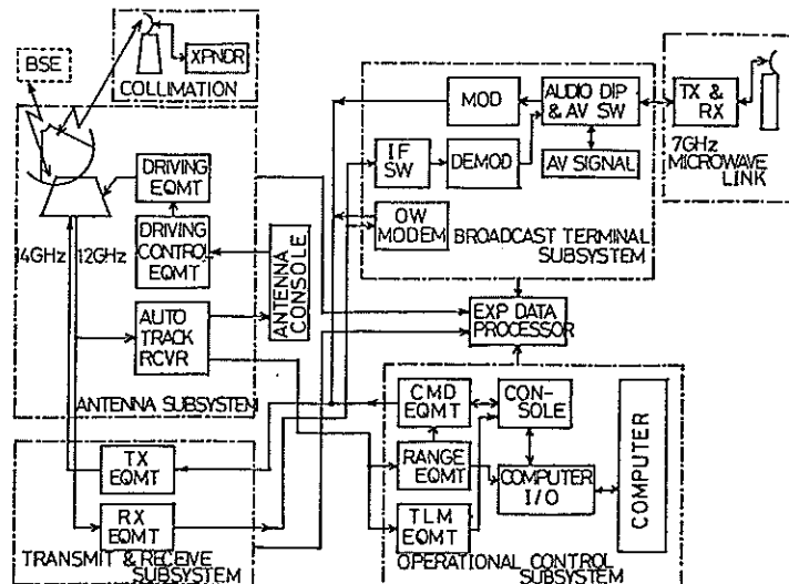
Fig. 4 Block diagram of Main Transmit & Receive Station
