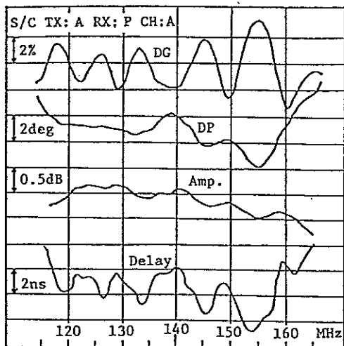
Fig. 5 Amplitude, delay, DG and DP characteristics of link
